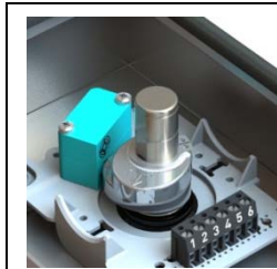
Fig. 3: Cam setting
