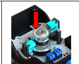
Fig. 2: Slot type cams
